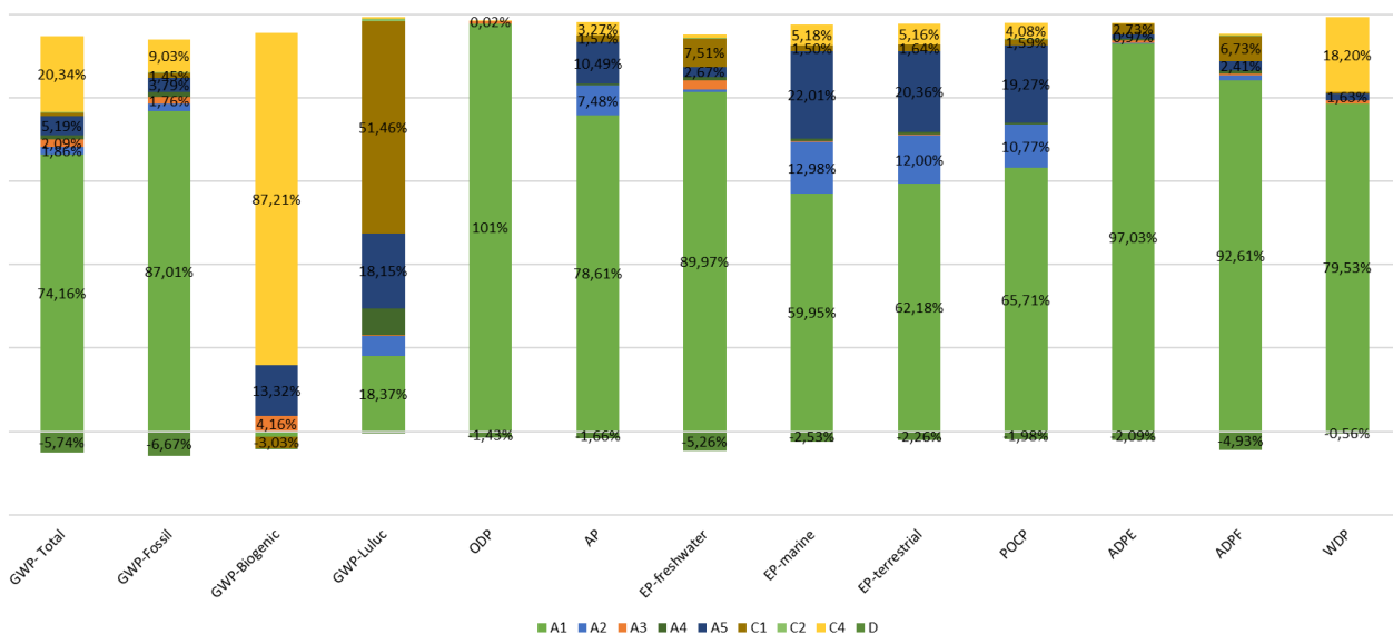
Domination analysis SAERTEX-LINER® ENVIRONMENT Ø 800 mm / 10 mm
