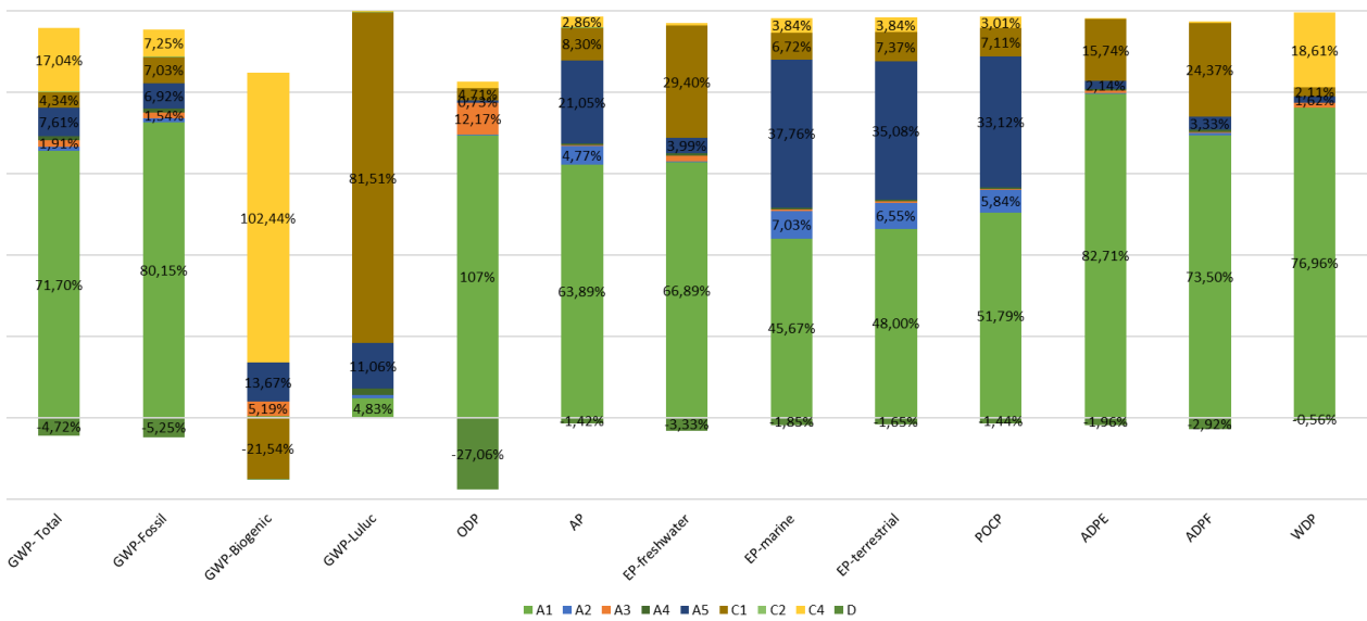
Dominanzanalyse SAERTEX-LINER® INDUSTRY Ø 300 mm / 3 mm
