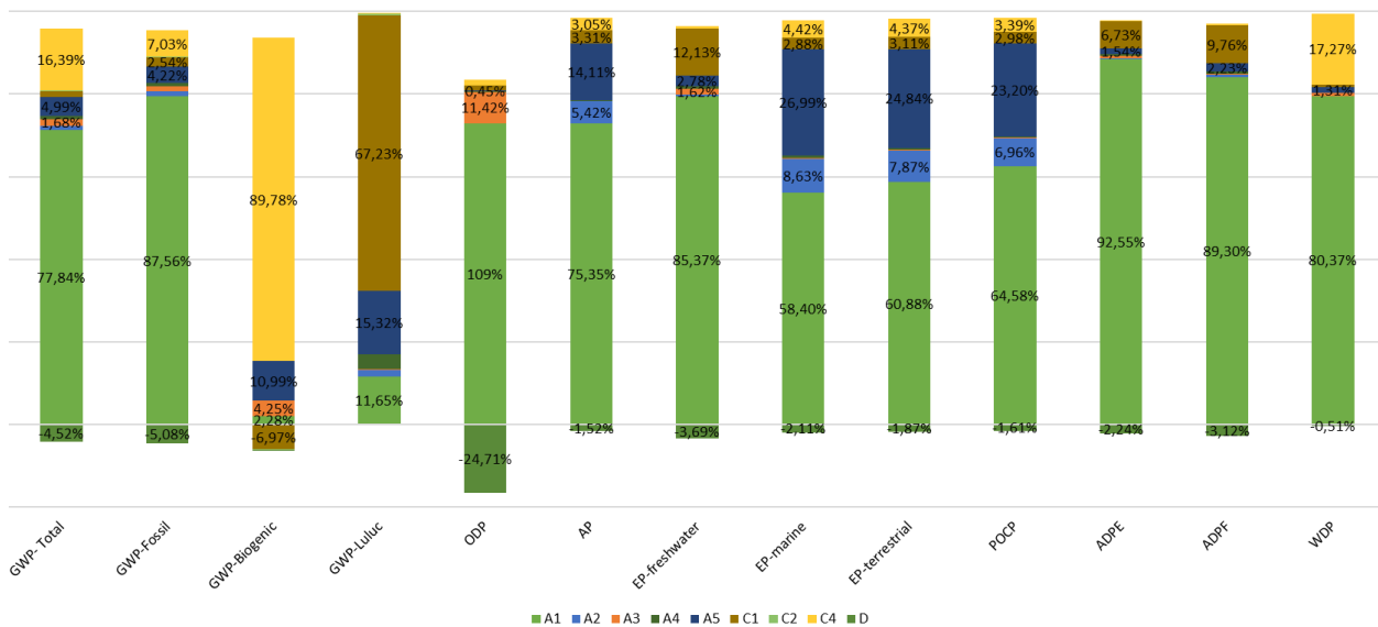
Domination analysis SAERTEX-LINER® INDUSTRY Ø 600 mm / 5 mm
