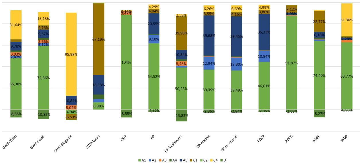
Domination analysis SAERTEX-LINER® GAS Ø 600 mm / 5,3 mm
