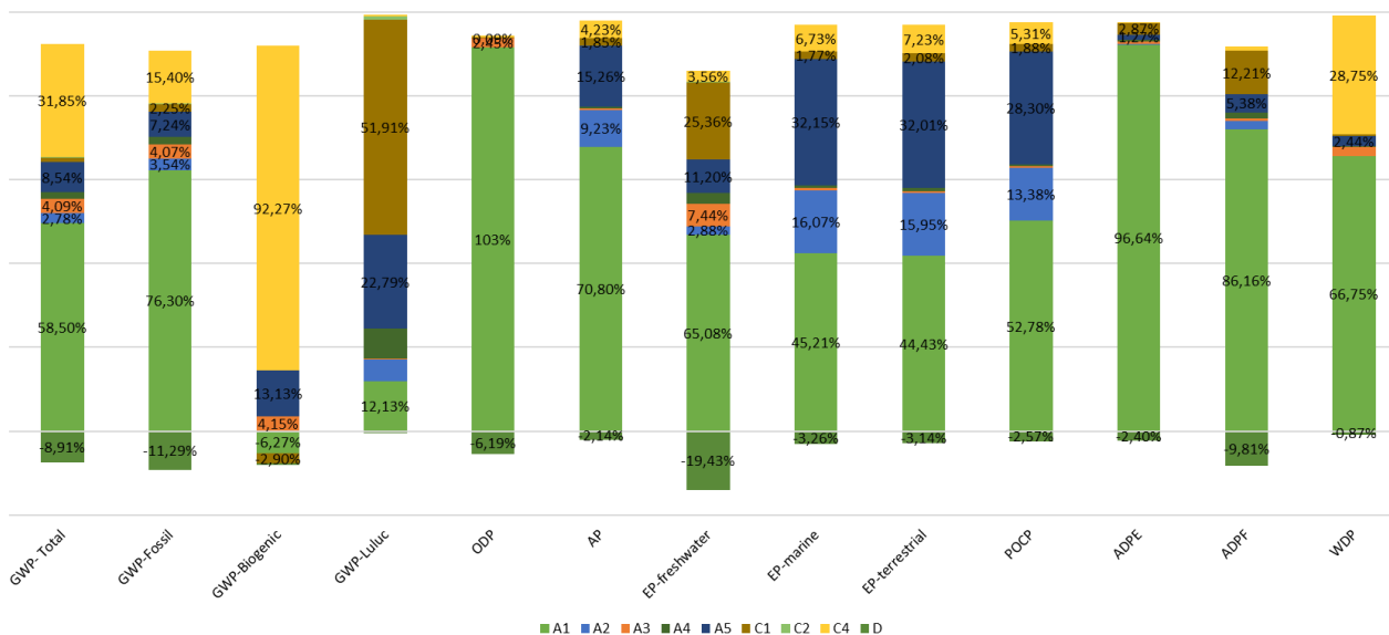
Domination analysis SAERTEX-LINER® GAS Ø 800 mm / 10,3 mm
